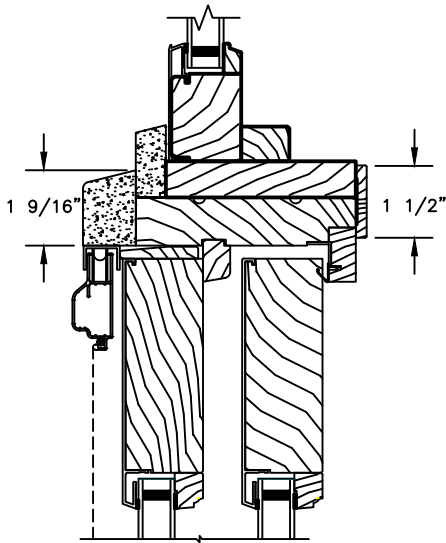
HORIZONTAL MULLION RADIUS/OPERATOR
