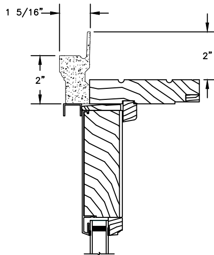
HEAD JAMB WITH 180 FLANGED BRICKMOULD
