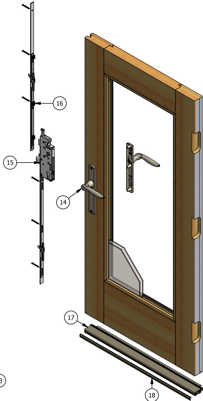
ACTIVE PANEL INTERIOR VIEW
