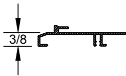
3/8" CLAD BRICKMOULD SUBSILL EXTRUSION
