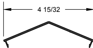
45° OUTSIDE MULL P.N.: 481018 LINEAL LENGTHS: 14'
