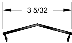
30° OUTSIDE MULL P.N.: 480021 LINEAL LENGTHS: 14'
