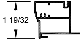
CLAD SQUARE BRICKMOULD EXTRUSION
