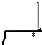
VINYL DRIP CAP (HINGED) P.N.: 471005 LINEAL LENGTH: 14'
