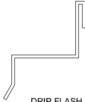
DRIP FLASH
