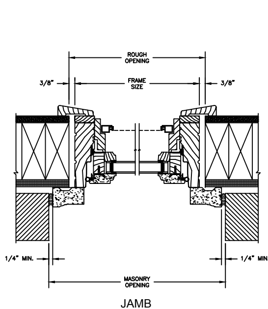
2 X 4 FRAME WITH BRICK VENEER
