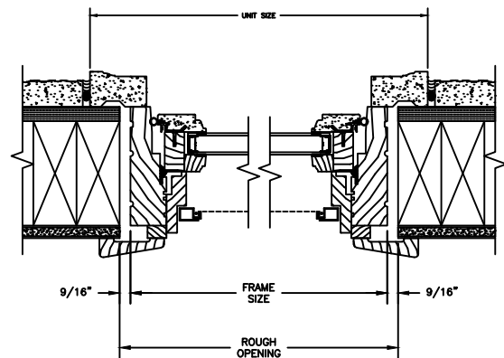
JAMBS 2 X 4 FRAME WITH STUCCO
