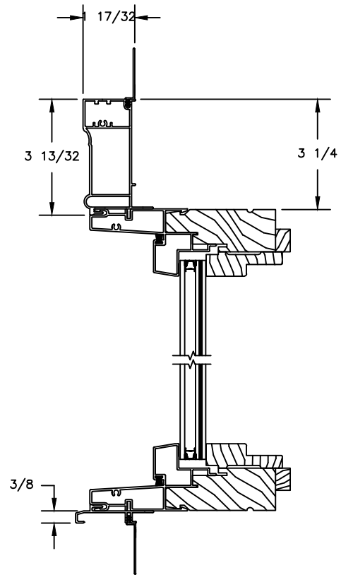
HEAD JAMB & SILL WITH CLAD WILLIAMSBURG CASING
