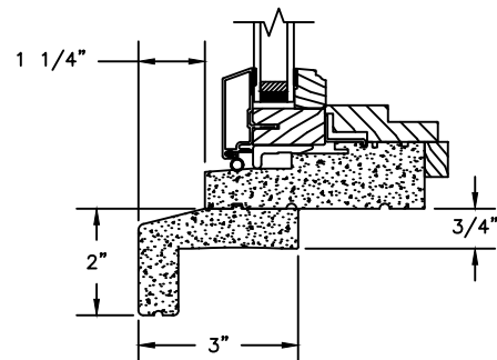
2" SUBSILL
