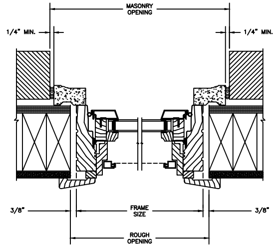
JAMB 2 X 4 FRAME WITH BRICK VENEER
