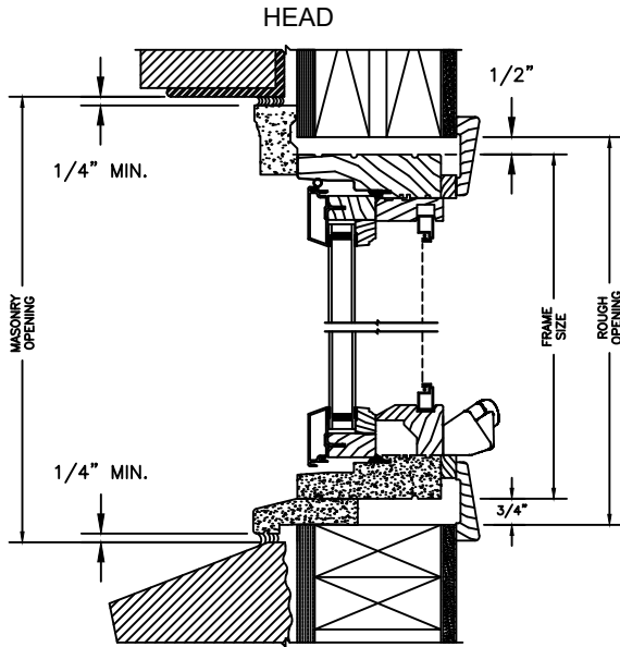
2 X 4 FRAME WITH BRICK VENEER HEAD SILL
