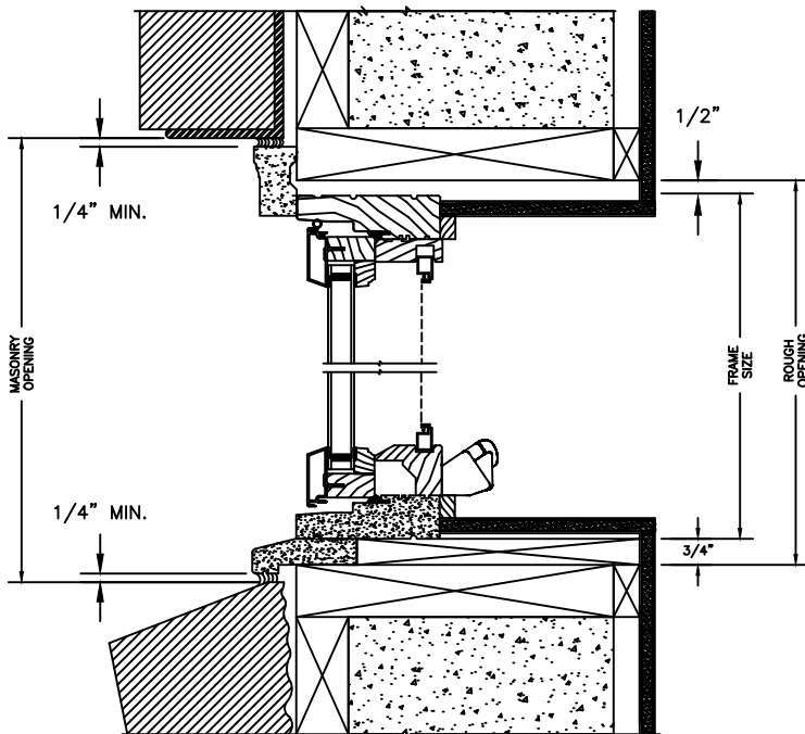
8" CONCRETEBLOCK WALL WITH BRICK VENEER HEAD SILL
