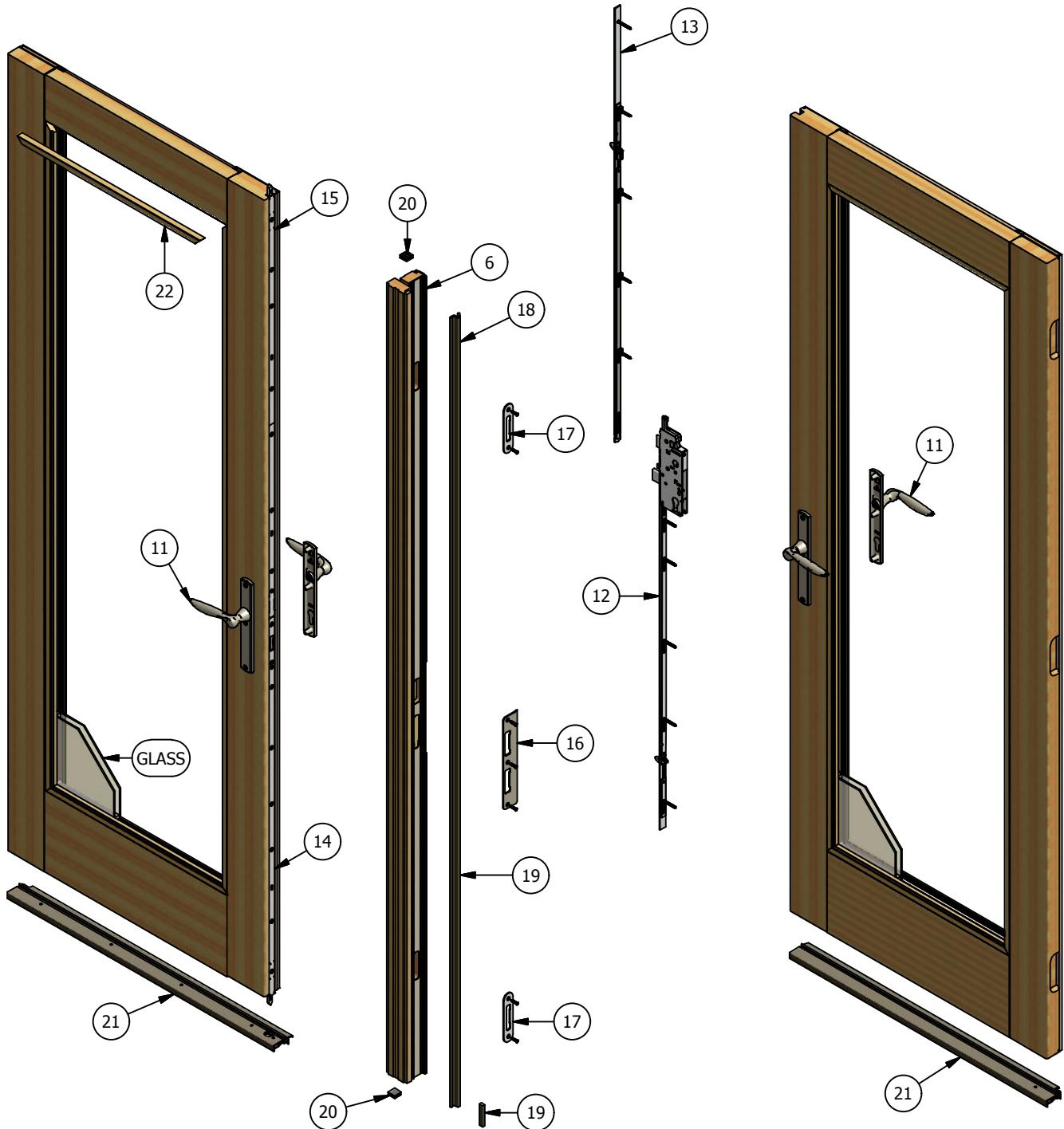
SECONDARY ACTIVE PANEL INTERIOR VIEW
