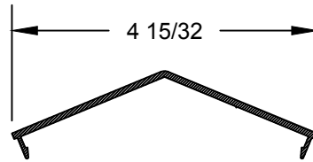
45° OUTSIDE MULL P.N.: 481018 LINEAL LENGTHS: 14'
