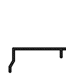
RIGID DRIP CAP P.N.: 483037 LENGTH: 14'
