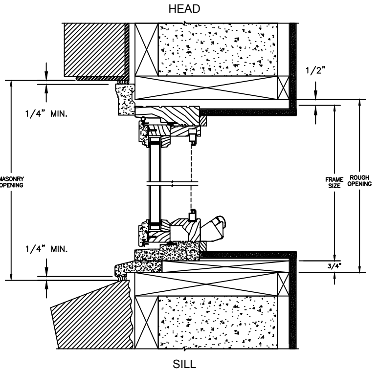
8" CONCRETE BLOCK WALL WITH BRICK VENEER
