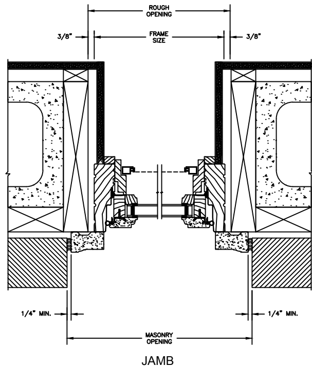
8" CONCRETE BLOCK WALL WITH BRICK VENEER
