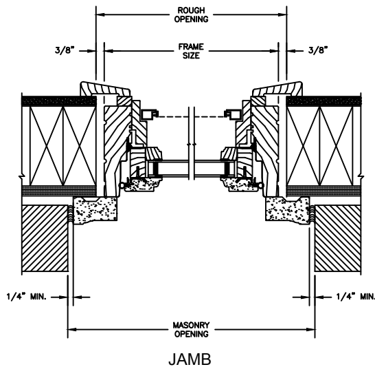
2 X 4 FRAME WITH BRICK VENEER
