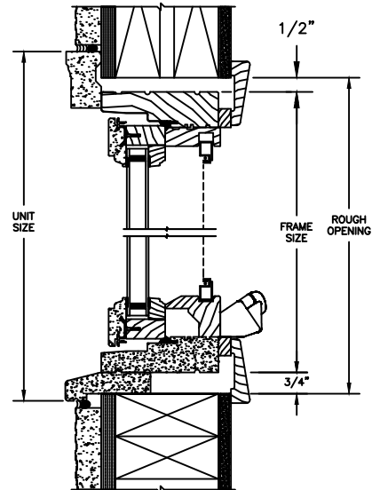
SILL 2 X 4 FRAME WITH STUCCO
