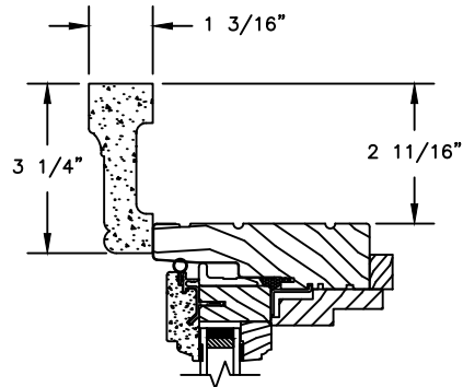
HEAD JAMB WITH WILLIAMSBURG BRICKMOULD
