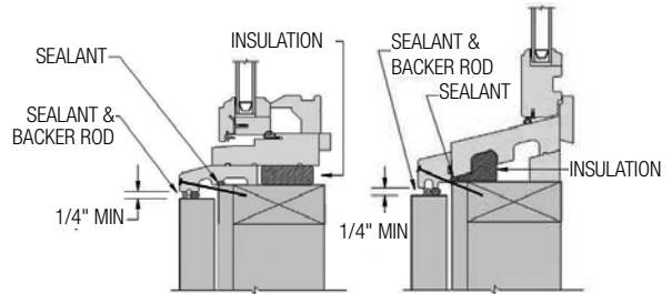
FIG. 17: DOUBLE HUNG SILL
