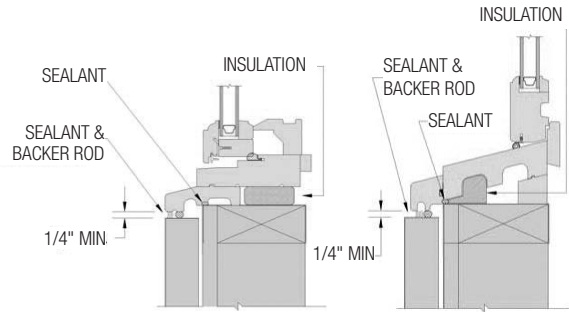
FIG. 16: CASEMENT SILL
