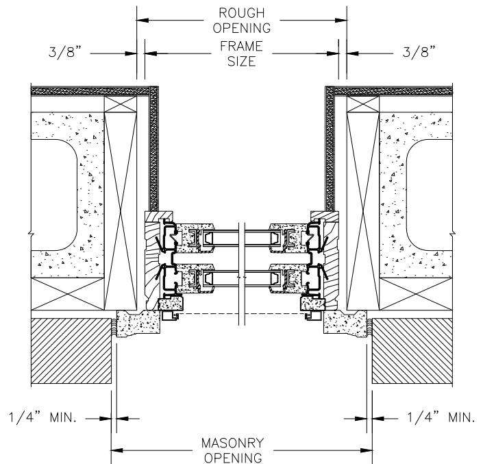
8" CONCRETE BLOCK WALL WITH BRICK VENEER
