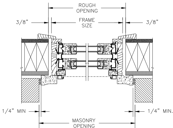
2 X 4 FRAME WITH BRICK VENEER
