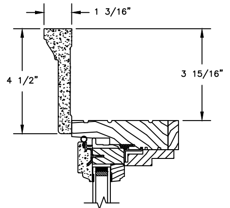
HEAD JAMB WITH 4 1/2" BACKBAND
