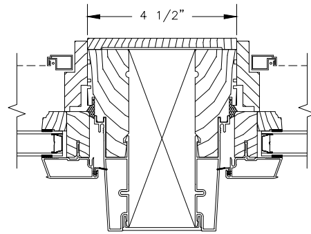
VERTICAL MULLION WITH 2" SPREAD MULL ADDITIONAL WIDTHS INCLUDE: 2 1/2", 4" & 6"
