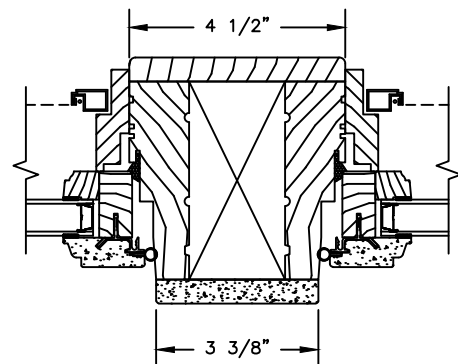
VERTICAL MULLION WITH 2" SPREAD MULL OPERATOR/OPERATOR
