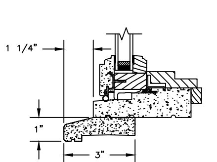
SILL WITH STANDARD SUBSILL
