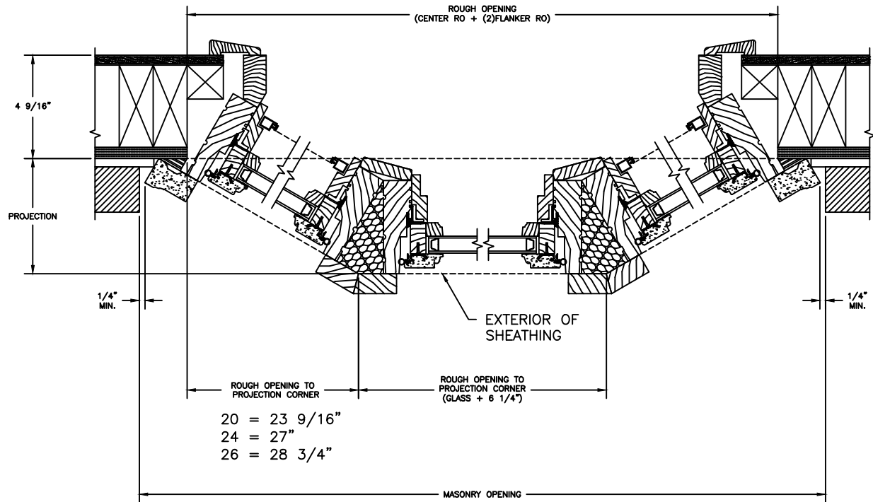
30 DEGREE BAY
