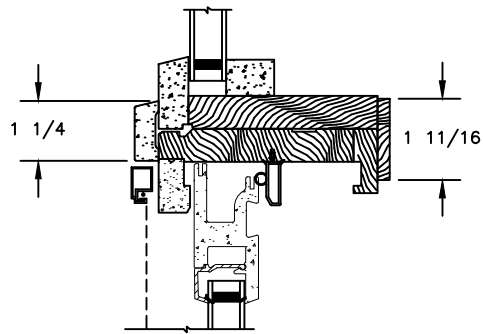
HORIZONTAL MULLION
