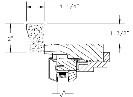
HEAD JAMB WITH WM180 BRICKMOULD
