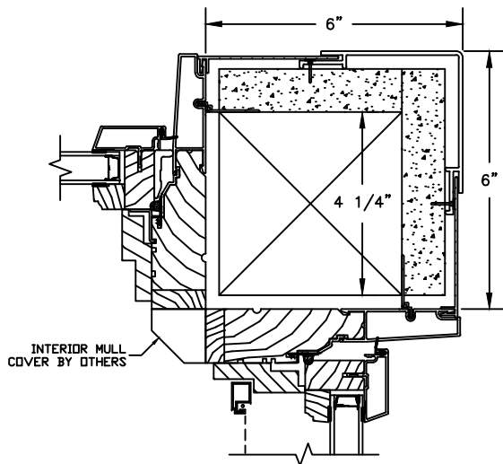
90° MULLION PICTURE/OPERATOR (ONLY USED WITH 4 9/16" JAMB & 3 1/4" FRAME EXPANDER)
