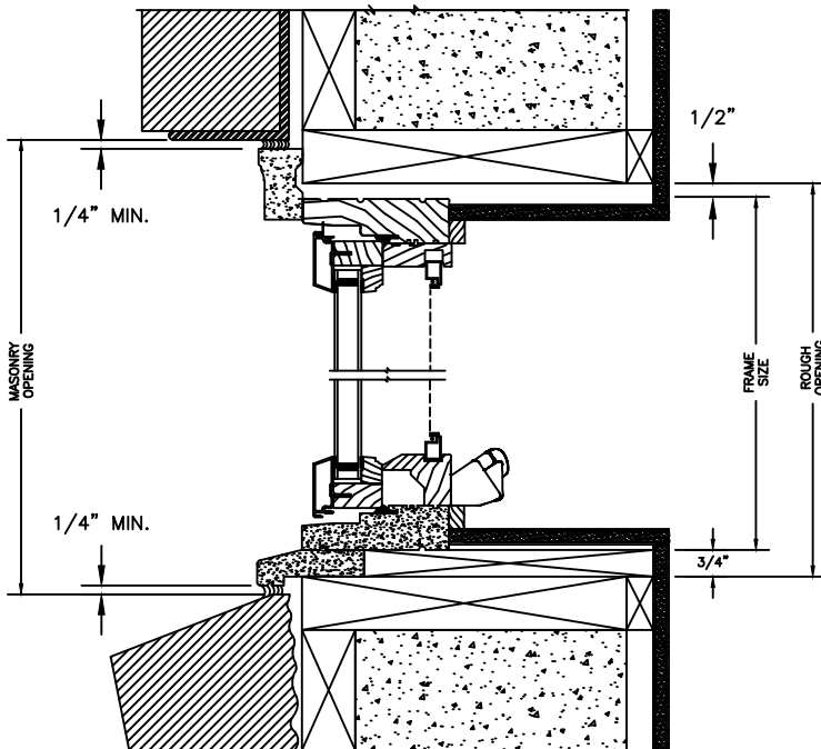
2 X 4 FRAME WITH BRICK VENEER HEAD
