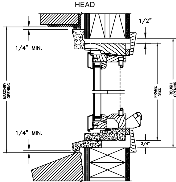
2 X 4 FRAME WITH BRICK VENEER HEAD
