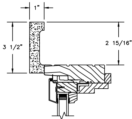
HEAD JAMB WITH 3 1/2" FLAT CASING
