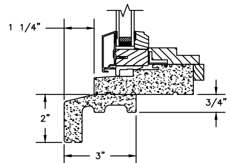
2" SUBSILL
