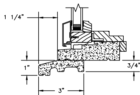
STANDARD SUBSILL
