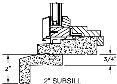
2" SUBSILL
