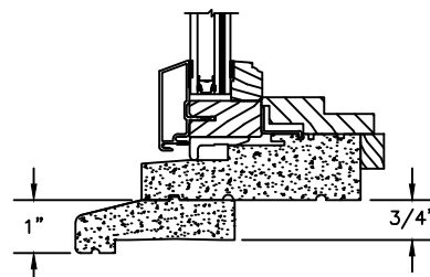
STANDARD SUBSILL
