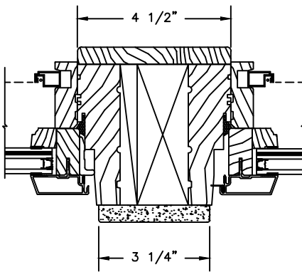
2" STRUCTURAL MULLION BY OTHERS
