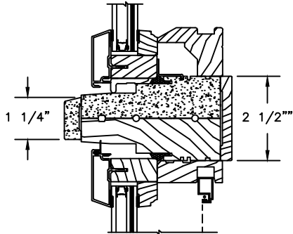
HORIZONTAL MULLION STATIONARY/OPERATOR
