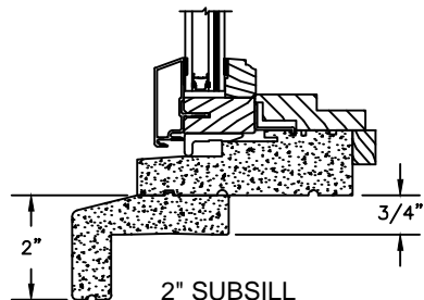
2" SUBSILL
