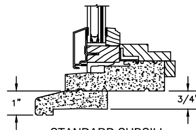
STANDARD SUBSILL
