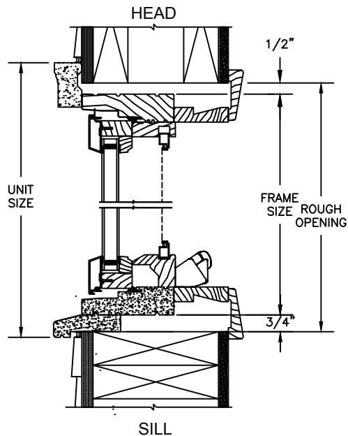
2 X 6 FRAME WITH SIDING
