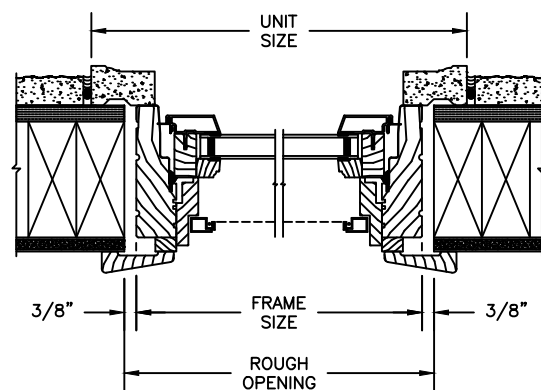
JAMB 2 X 4 FRAME WITH STUCCO
