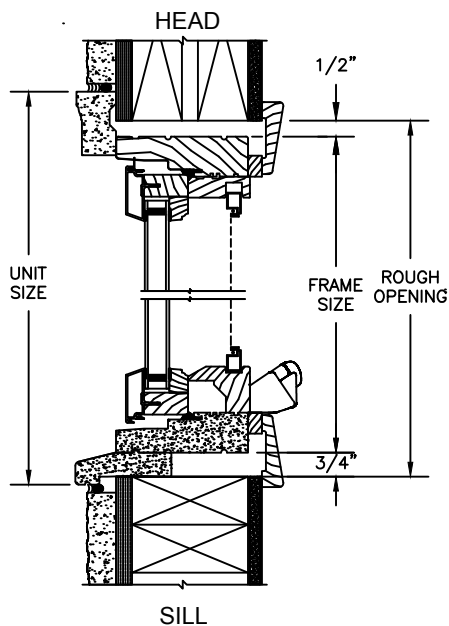
2 X 4 FRAME WITH STUCCO
