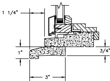
STANDARD SUBSILL
