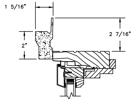
HEAD JAMB WITH 180 FLANGED BRICKMOULD
