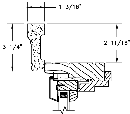
HEAD JAMB WITH WILLIAMSBURG BRICKMOULD
