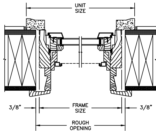
JAMB 2 X 6 FRAME WITH SIDING
