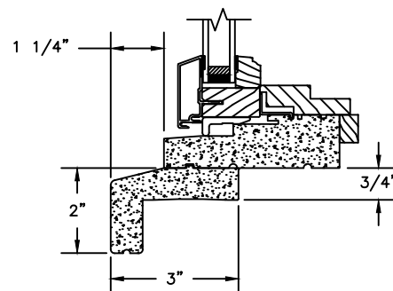
2" SUBSILL
