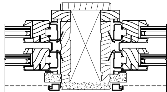
VERTICAL MULLION WITH 2" SPREAD MULL OPERATOR/OPERATOR ADDITIONAL WIDTHS INCLUDE: 1" - 5"
