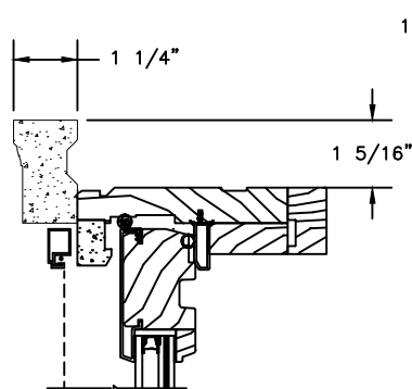
HEAD JAMB WITH WM180 BRICKMOULD
