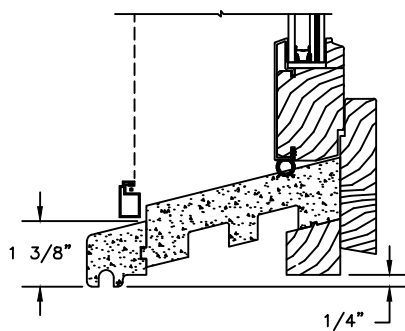
STANDARD SILLNOSE
