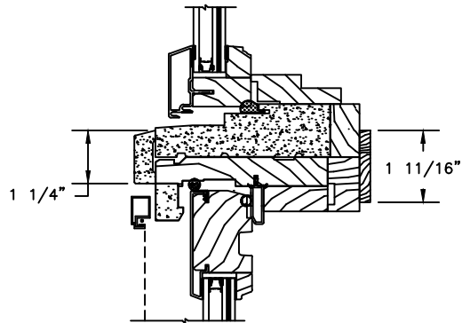
HORIZONTAL MULLION TRANSOM/OPERATOR
