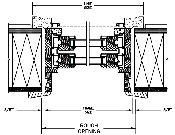
JAMB 2 X 6 FRAME WITH SIDING
