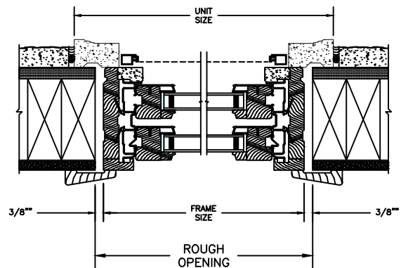
JAMB 2 X 4 FRAME WITH STUCCO
