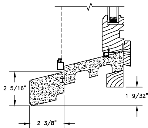
BELLY SUBSILL
