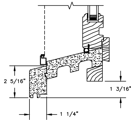
BULLNOSE SUBSILL
