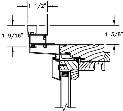
HEAD JAMB WITH CLAD 180 BRICKMOULD CASING
