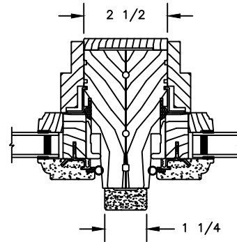
VERTICAL MULLION STATIONARY/STATIONARY
