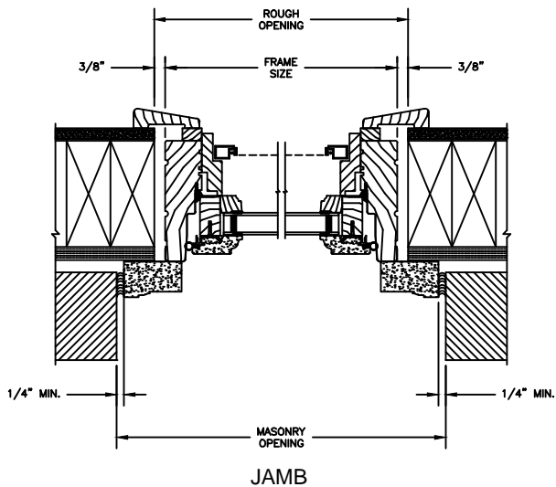
2 X 4 FRAME WITH BRICK VENEER
