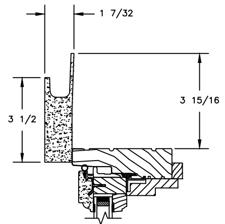
HEAD JAMB WITH 3 1/2" FLAT CASING WITH J-CHANNEL
