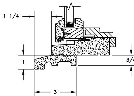
SILL WITH STANDARD SUBSILL
