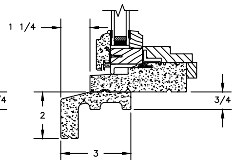
SILL WITH 2" SUBSILL
