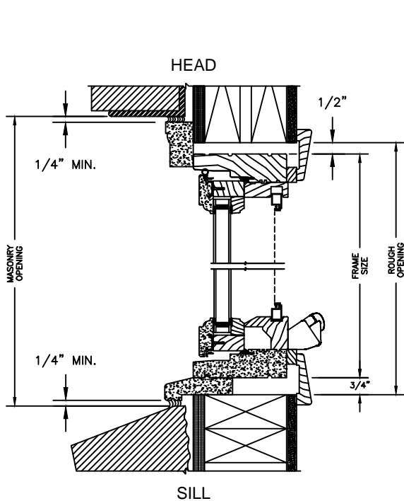
2 X 4 FRAME WITH BRICK VENEER
