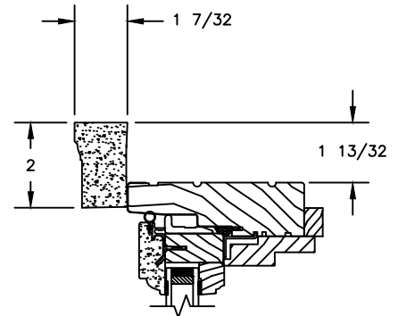
HEAD JAMB WITH WM180 BRICKMOULD
