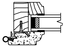
OGEE GLASS STOP
