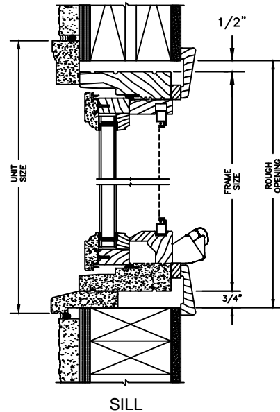
2 X 4 FRAME WITH STUCCO
