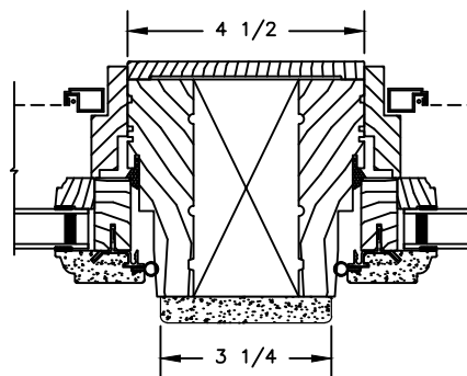
VERTICAL MULLION OPERATOR WITH 2" SPREAD MULL
