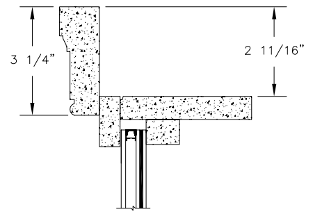
HEAD JAMB WITH WILLIAMSBURG BRICKMOULD
