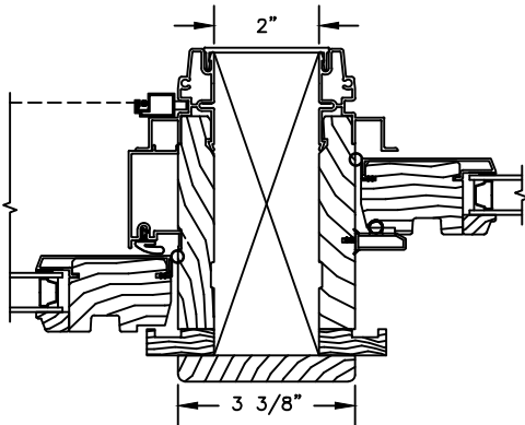
VERTICAL MULLION WITH 2" SPREAD MULL OPERATOR/OPERATOR
