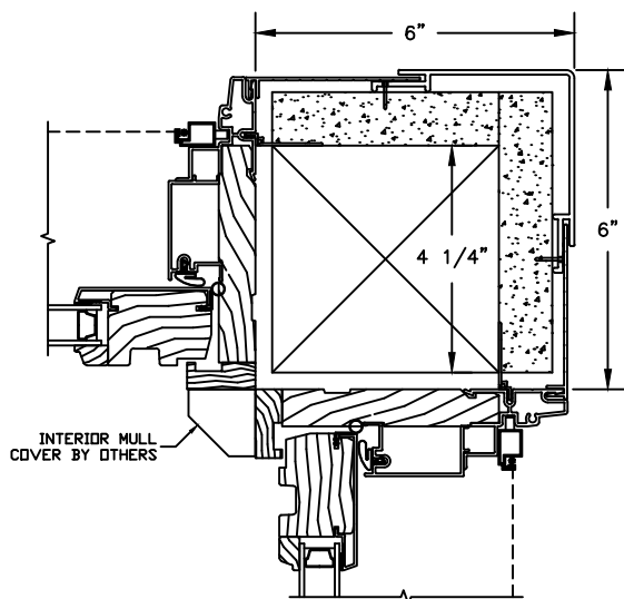
90° MULLION OPERATOR/OPERATOR
