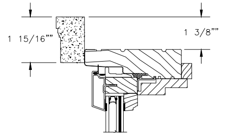
HEAD JAMB WITH WM180 BRICKMOULD
