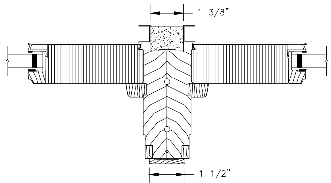
VERTICAL MULLION STATIONARY/STATIONARY
