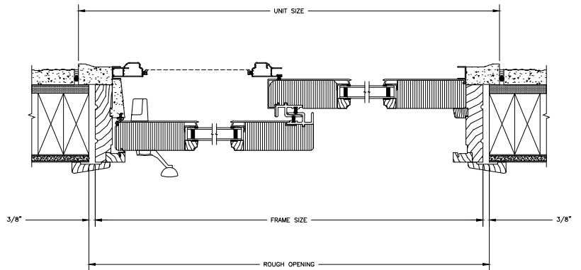
JAMBS 2 X 4 FRAME WITH STUCCO
