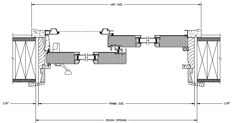
JAMBS 2 X 6 FRAME WITH SIDING
