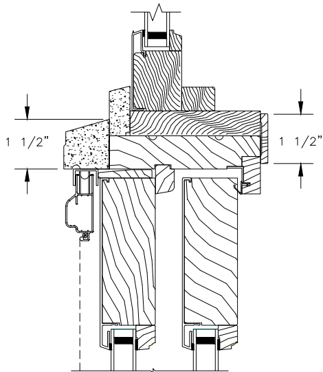
HORIZONTAL MULLION RADIUS/OPERATOR
