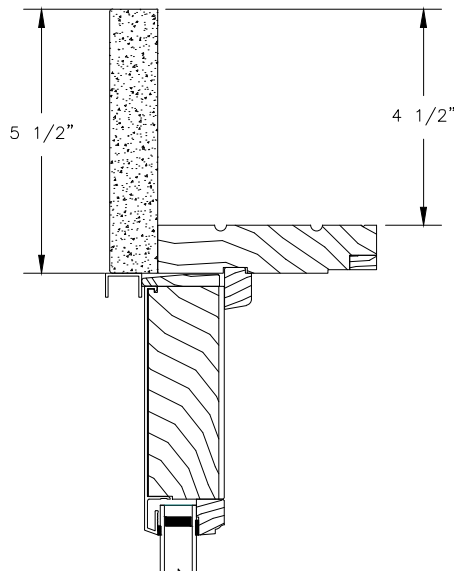
HEAD JAMB WITH 5 1/2" FLAT CASING
