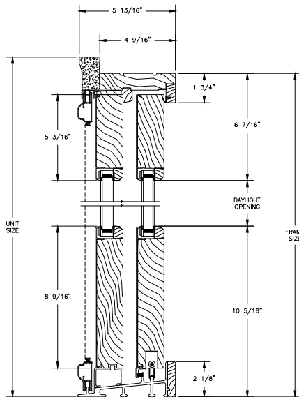
OPERATING HEAD JAMB & SILL
