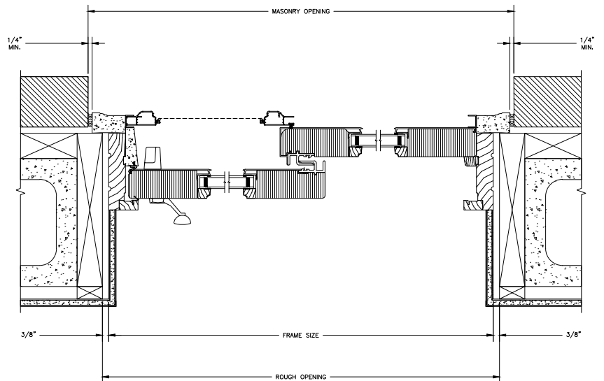
JAMBS 8" CONCRETE BLOCK WALL WITH BRICK VENEER
