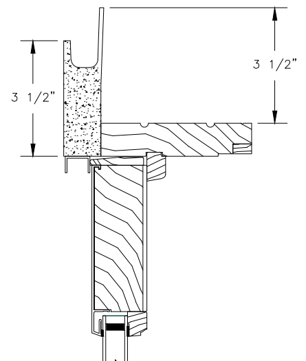
HEAD JAMB WITH 3 1/2" FLAT CASING WITH J-CHANNEL
