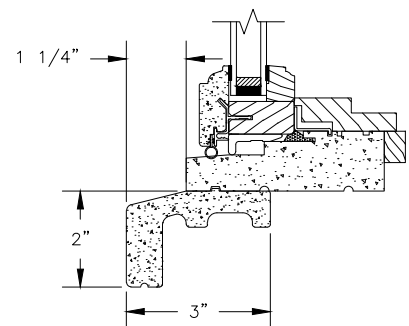
SILL WITH 2" SUBSILL
