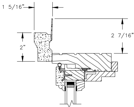
HEAD JAMB WITH 180 FLANGED BRICKMOULD
