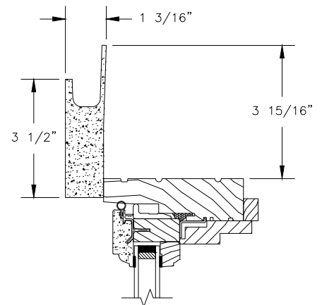
HEAD JAMB WITH 3 1/2" FLAT CASING WITH J-CHANNEL
