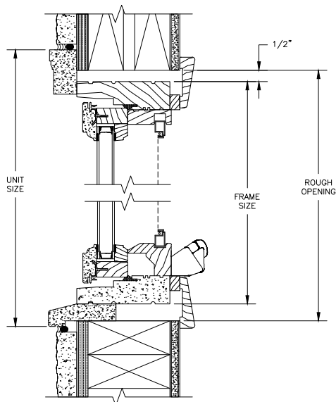
HEAD JAMB & SILL 2 X 4 FRAME WITH STUCCO
