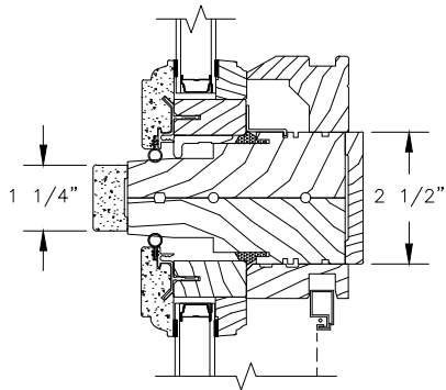
HORIZONTAL MULLION STATIONARY/OPERATOR
