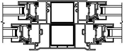
VERTICAL T-BAR OPERATOR/OPERATOR
