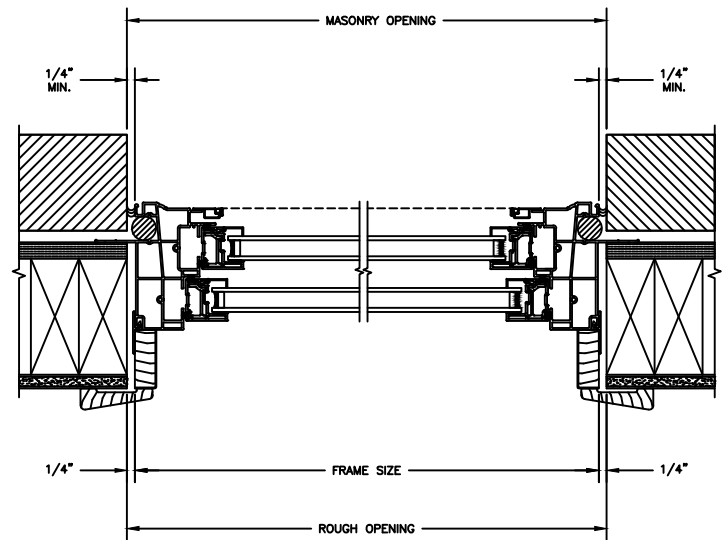
JAMBS 2 X 4 FRAME WITH BRICK VENEER
