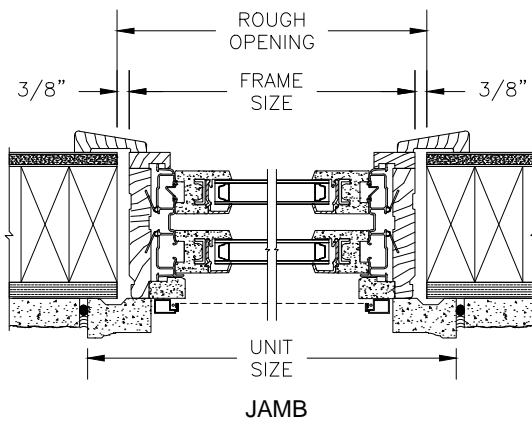
2 X 4 FRAME WITH STUCCO
