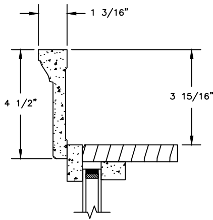
HEAD JAMB WITH 4 1/2" BACKBAND
