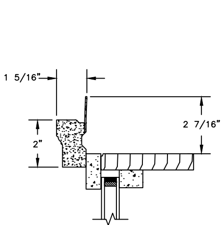
HEAD JAMB WITH 180 FLANGED BRICKMOULD
