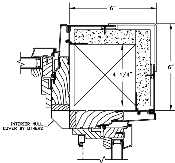
90° MULLION PICTURE/OPERATOR
