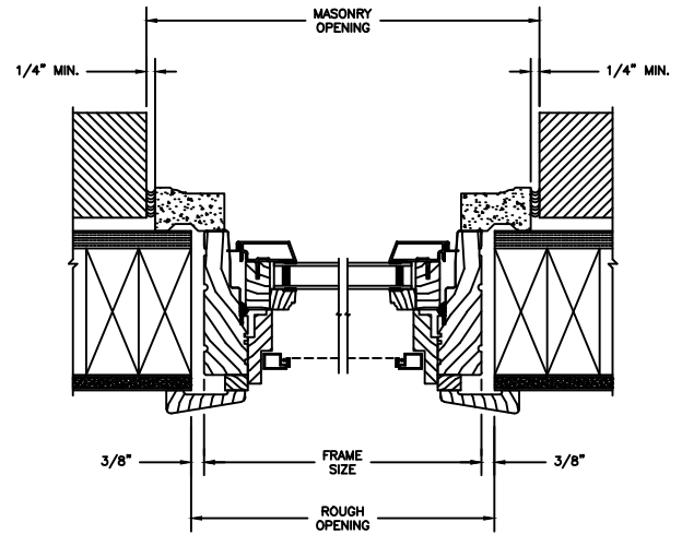
JAMB 2 X 4 FRAME WITH BRICK VENEER
