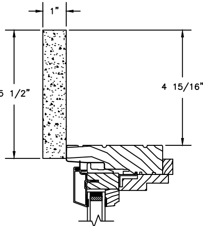
HEAD JAMB WITH 5 1/2" FLAT CASING
