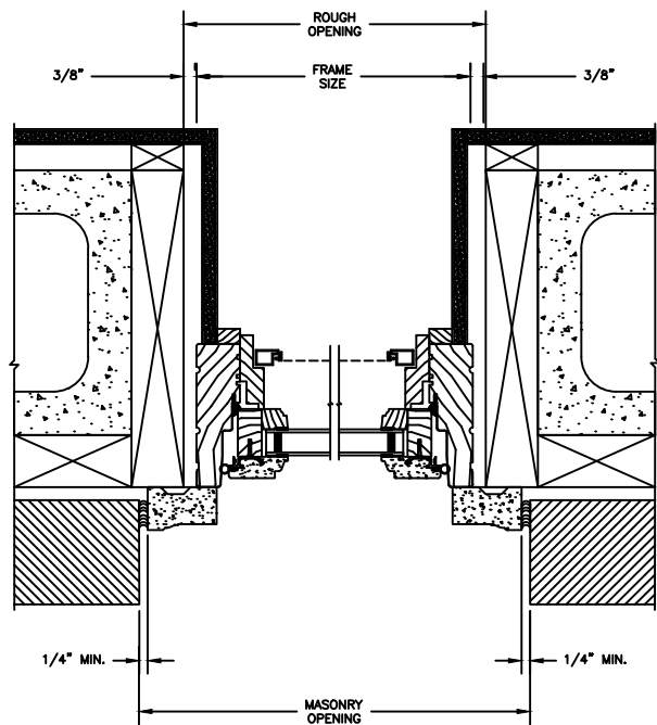
JAMB 8" CONCRETE BLOCK WALL WITH BRICK VENEER
