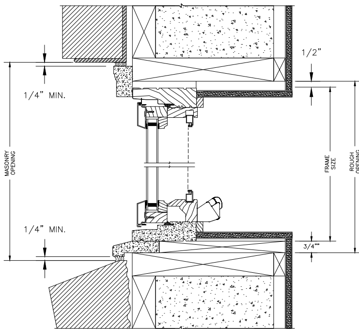
8" CONCRETEBLOCK WALL WITH BRICK VENEER
