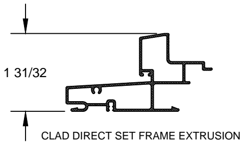
CLAD DIRECT SET FRAME EXTRUSION
