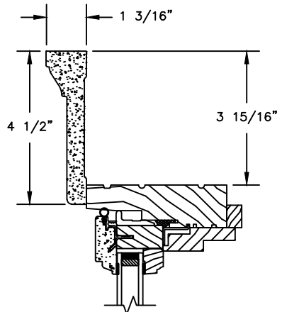
HEAD JAMB WITH 4 1/2" BACKBAND
