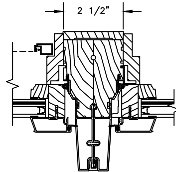
VERTICAL MULLION OPERATOR/STATIONARY
