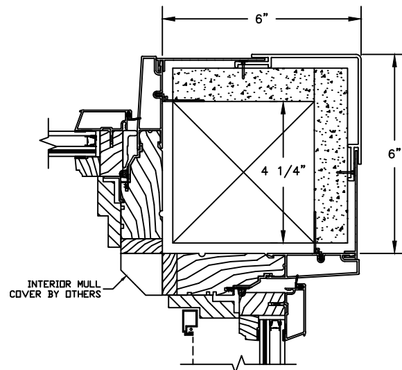
90° MULLION STATIONARY/OPERATOR
