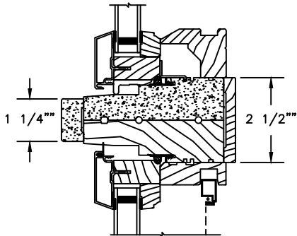
HORIZONTAL MULLION STATIONARY/OPERATOR
