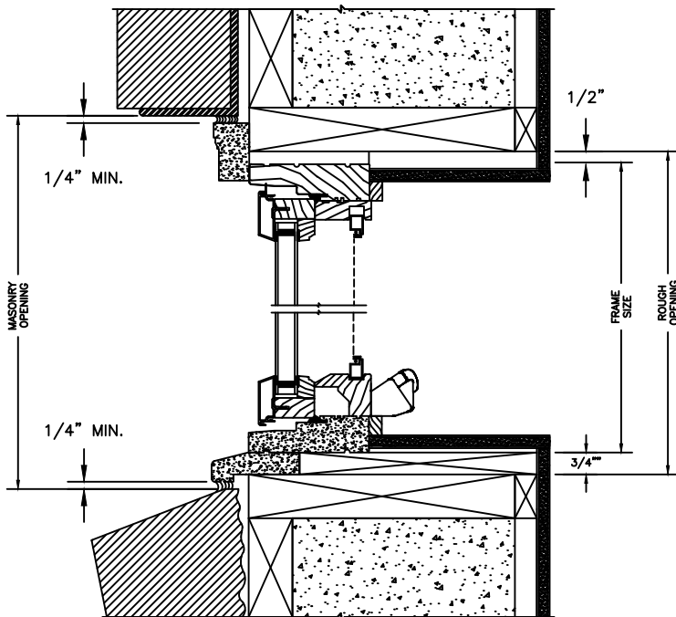
SILL 8\" CONCRETEBLOCK WALL WITH BRICK VENEER
