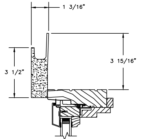
HEAD JAMB WITH 3 1/2" FLAT CASING WITH J-CHANNEL
