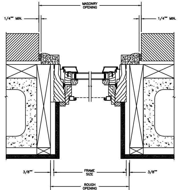
JAMB 8\" CONCRETE BLOCK WALL WITH BRICK VENEER
