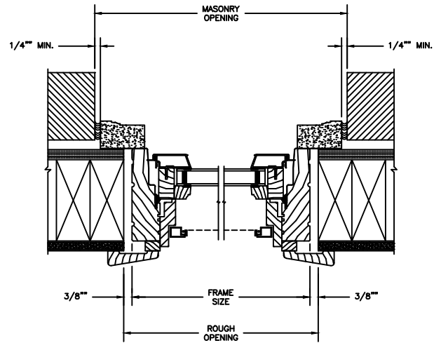
JAMB 2 X 4 FRAME WITH BRICK VENEER
