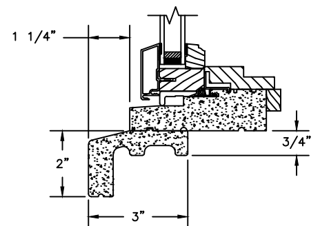
2" SUBSILL
