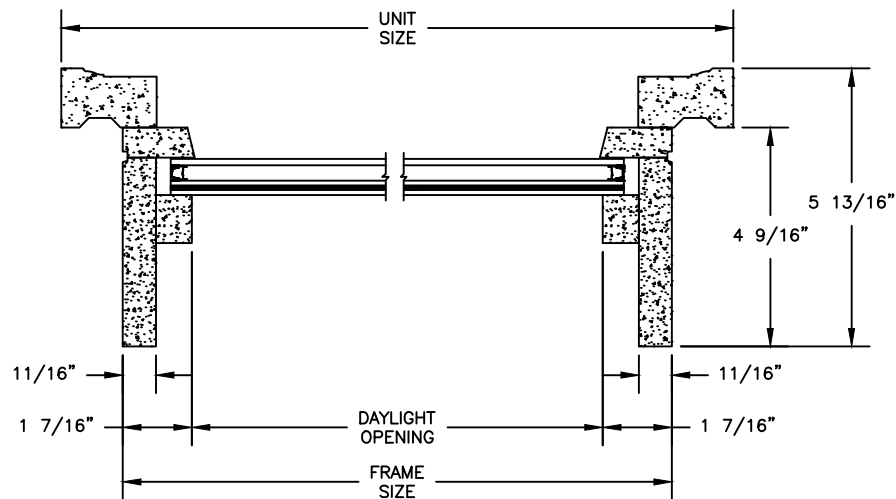
HALF ROUNDS, FULL ROUNDS & OVALS JAMB
