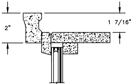
HEAD JAMB WITH STANDARD 180 BRICKMOULD
