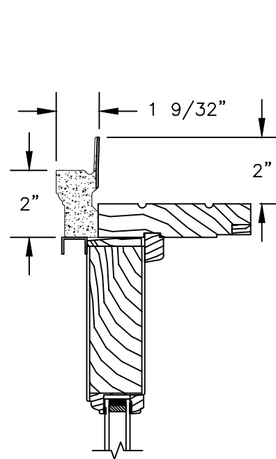
HEAD JAMB WITH 180 FLANGED BRICKMOULD
