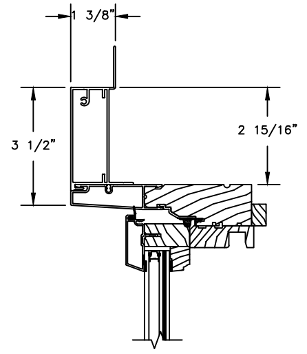
HEAD JAMB WITH 3 1/2" CLAD FLAT CASING
