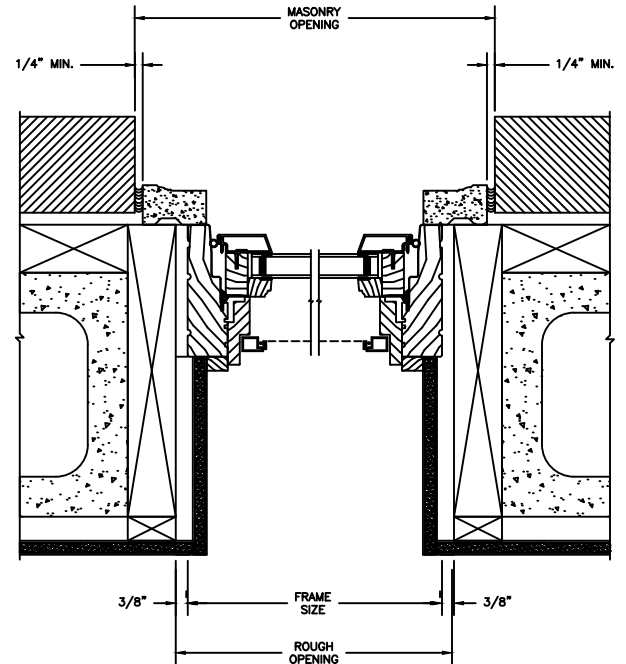
JAMB 8" CONCRETE BLOCK WALL WITH BRICK VENEER
