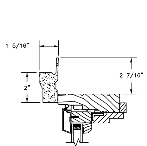
HEAD JAMB WITH 180 FLANGED BRICKMOULD
