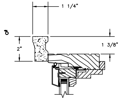
HEAD JAMB WITH WM180 BRICKMOULD
